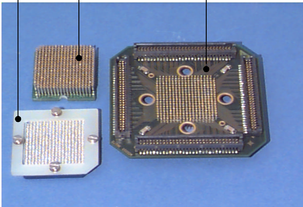
E-Tec Socket, Emulation Technology BGA Block, Lauterbach Adapter (Top view)
