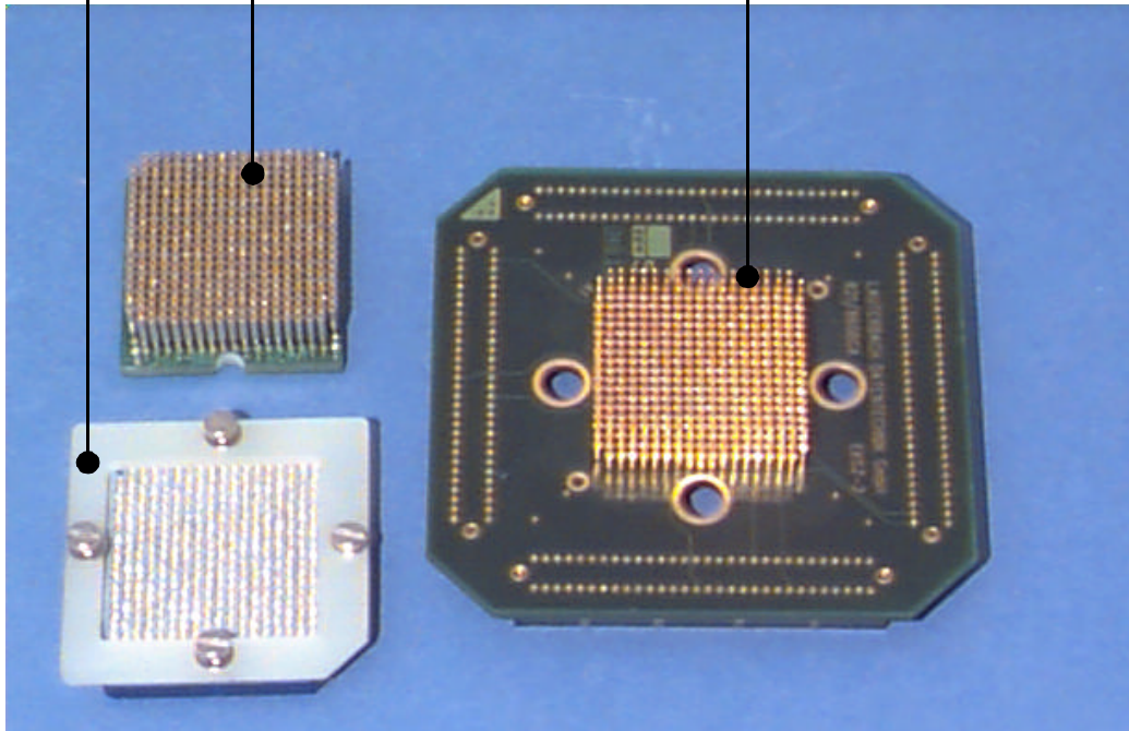
E-Tec Socket, Emulation Technology BGA Block, Lauterbach Adapter (Bottom view)
